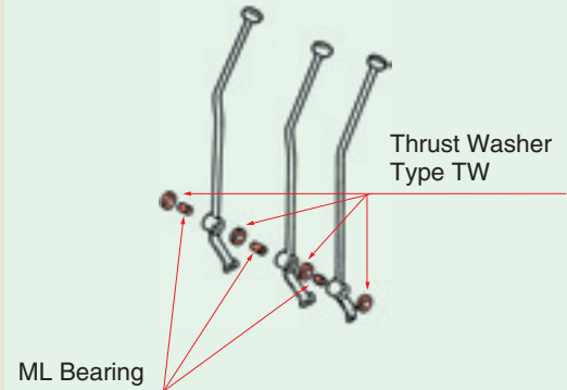
Control Lever for Construction Machine
