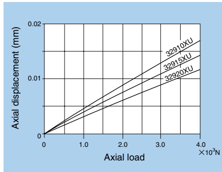
Fig. 9.6.2 Axial Load and Displacement for 329 Series
