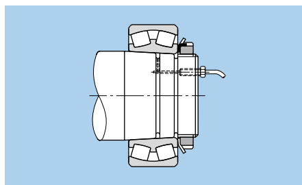
Fig. 16.5 Mounting by Oil Injection
