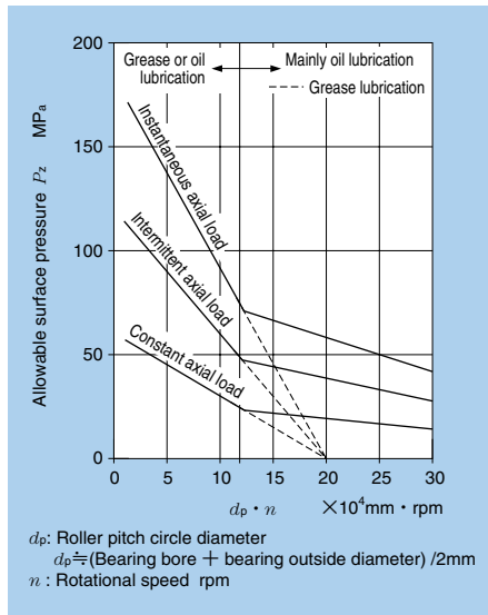
Fig. 7.7 Allowable Surface Pressure of Rib
