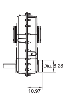
REDUCER WITH BACKSTOP
