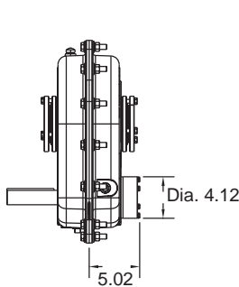
REDUCER WITH BACKSTOP
