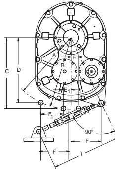
DOUBLE REDUCTION TORQUE-ARM REDUCERS
