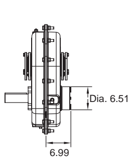
REDUCER WITH BACKSTOP
