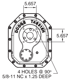
FLANGE MOUNTING DIMENSIONS
