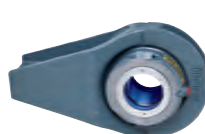
Rod End Shoe 1 3/16"/30mm to 6"/155mm Available in cast iron Also offered as tee type
