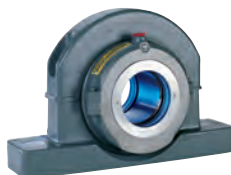
Pedestal Unit 1 3/16"/30mm to 24"/600mm Available in cast iron ductile iron or steel
