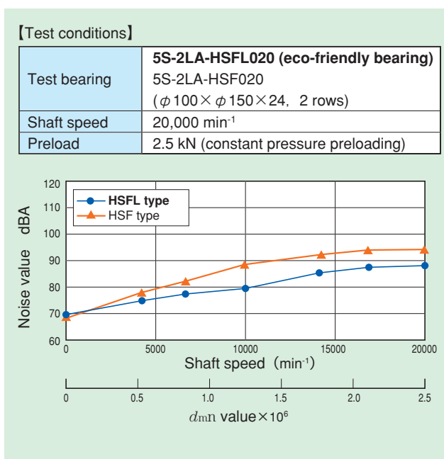
Fig. 8.11 Comparison of noise values
