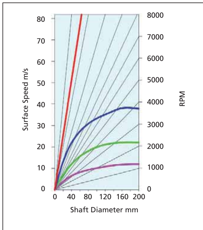
Figure 94 Surface speed as a function of shaft diameter and RPM
