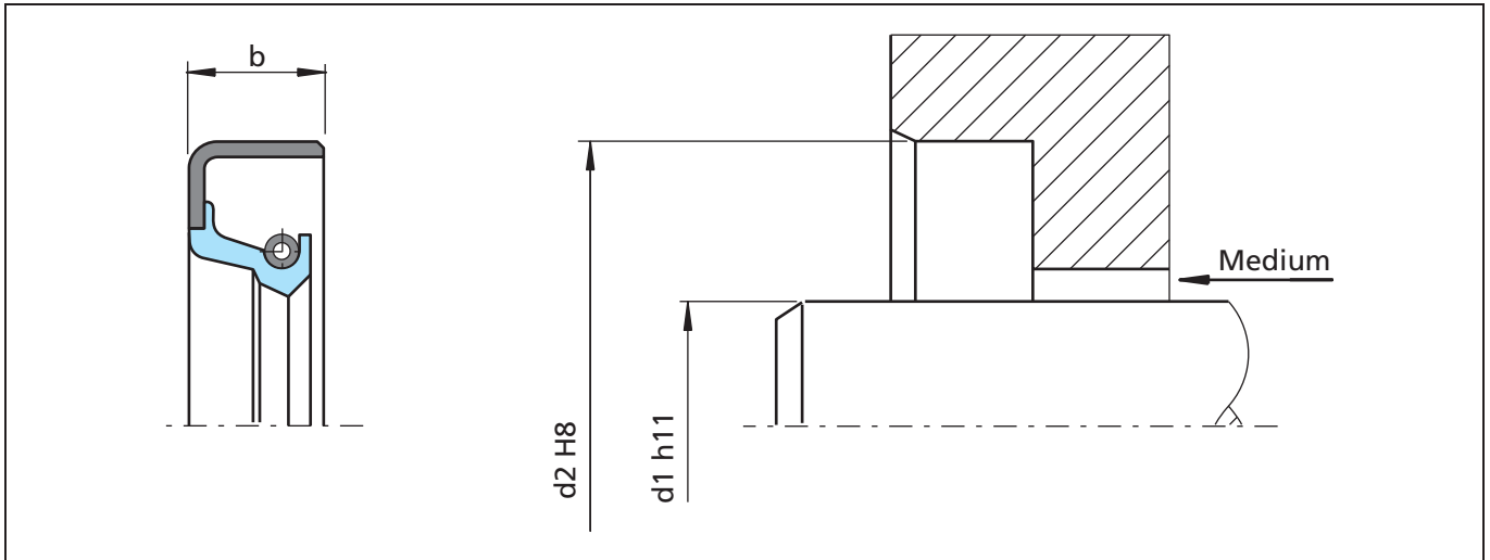
Figure 16 Installation drawing
