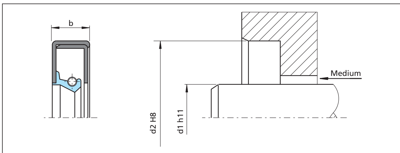
Figure 18 Installation drawing
