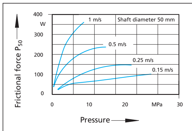
Figure 136 Frictional power for Turcon® Roto Variseal®
