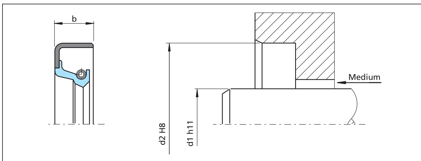
Figure 16 Installation drawing
