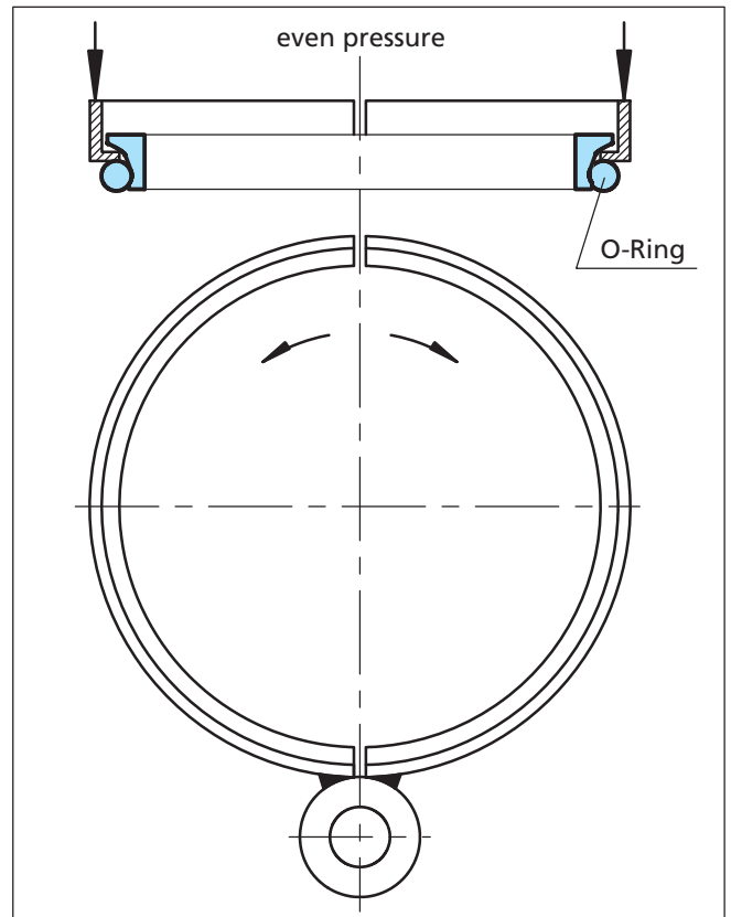
Figure 146 Fitting Tool
