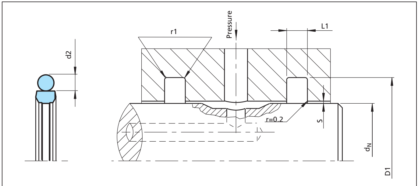
Figure 133 Installation drawing
