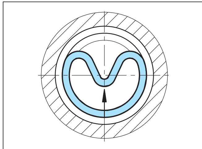
Figure 131 Inserting the seal ring into the closed groove
