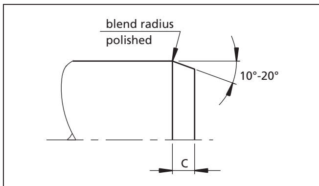
Figure 128 Lead-in chamfer on shaft
