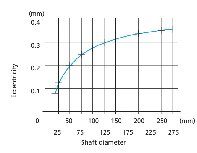
Figure 59 Permissible eccentricity
