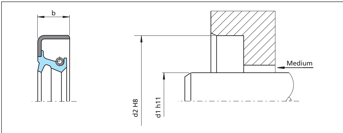
Figure 17 Installation drawing
